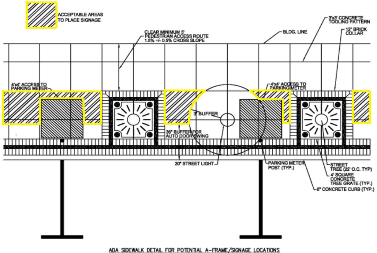
ADA SIDEWALK DETAIL FOR POTENTIAL A-FRAME/SIGNAGE LOCATIONS
